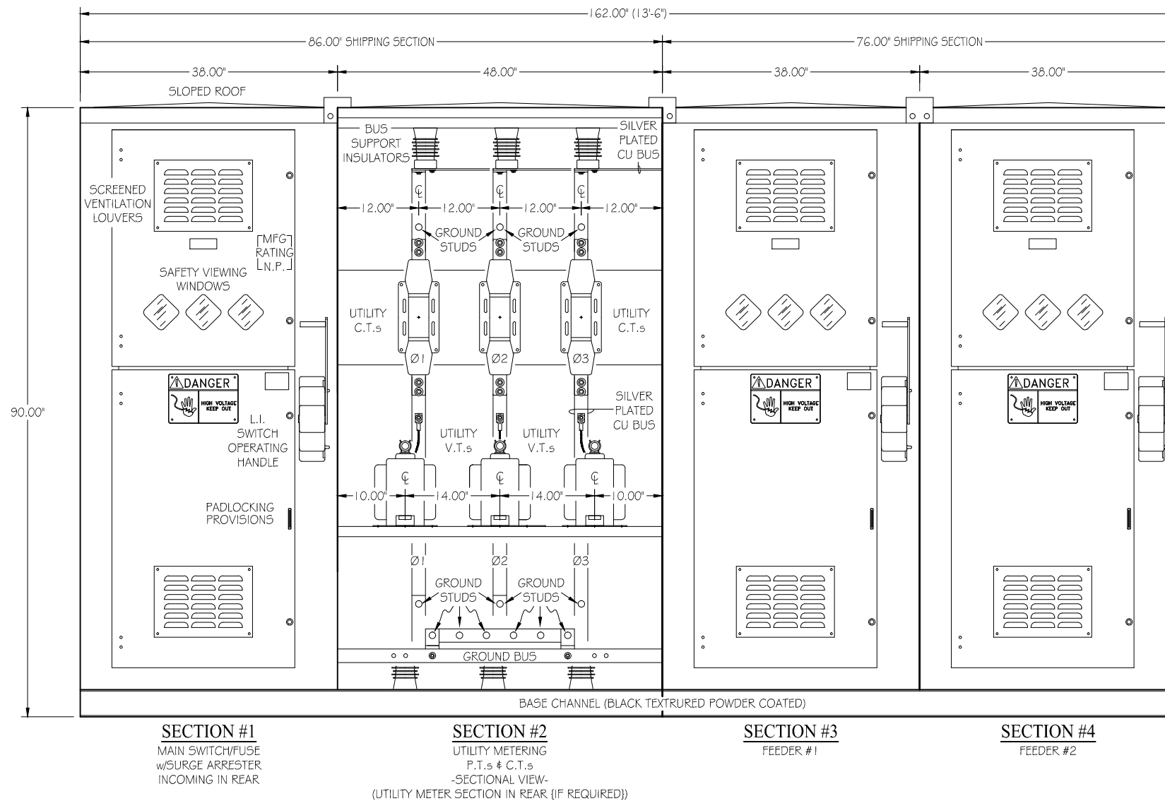
FRONT ELEVATION
