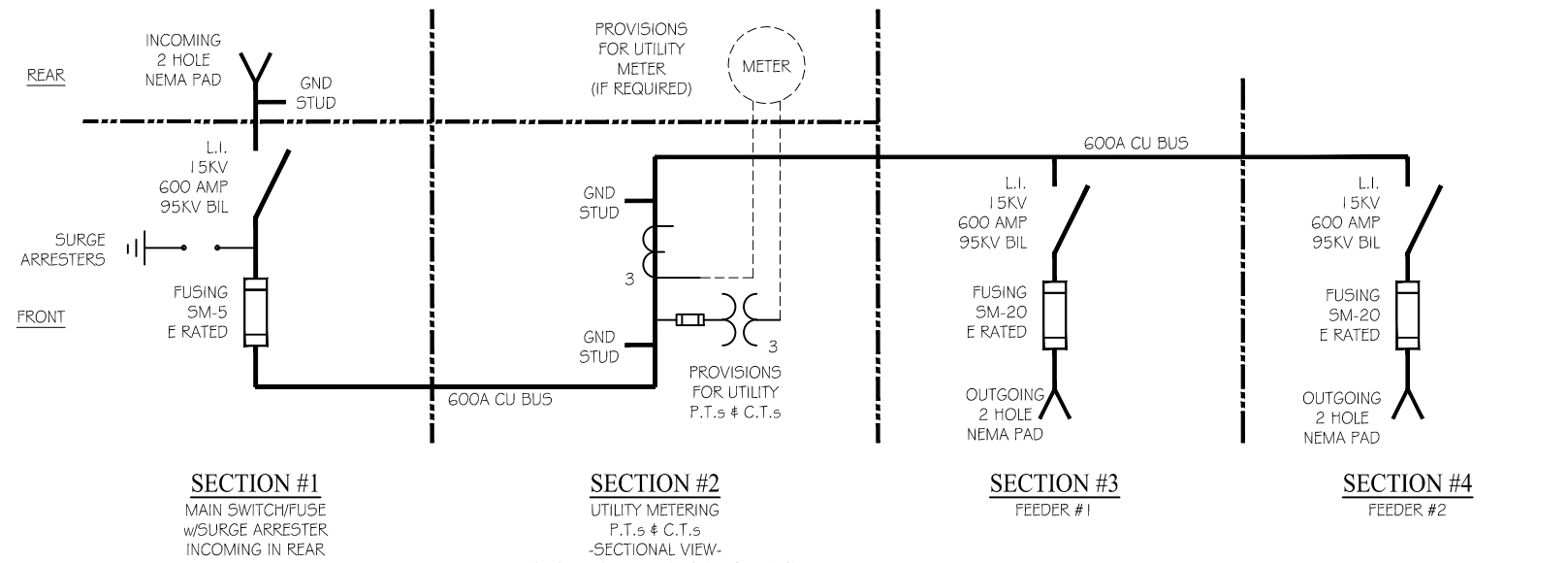
SINGLE LINE DIAGRAM
